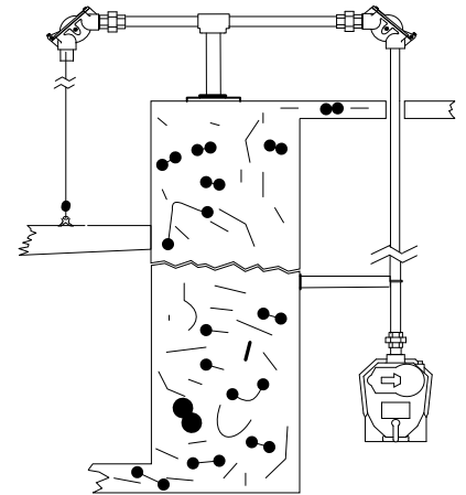
2579 DIGESTER COVER POSITION INDICATOR
