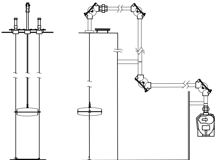
2582 EXTERNAL TANK DIKE GROUND READING
