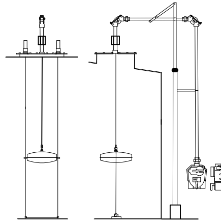
2578-HACC HIGH ACCURACY IN SERVICE KIT FOR CONE ROOF TANK
