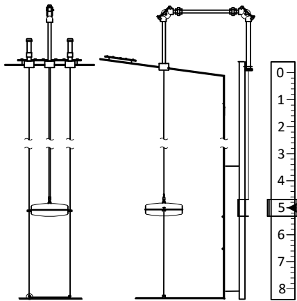
2582 EXTERNAL TANK DIKE GROUND READING
