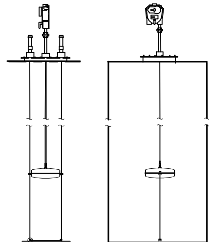
2583SK IN SERVICE KIT TOP MOUNTED (SUMP KIT)
