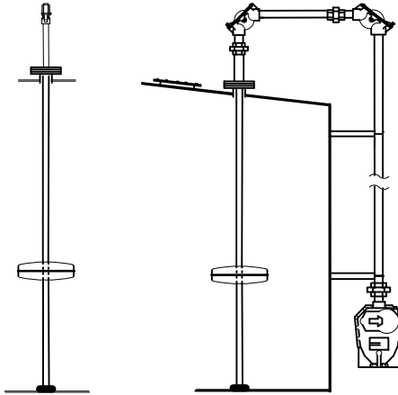
2580 MAGNETIC COUPLED GROUND READING
