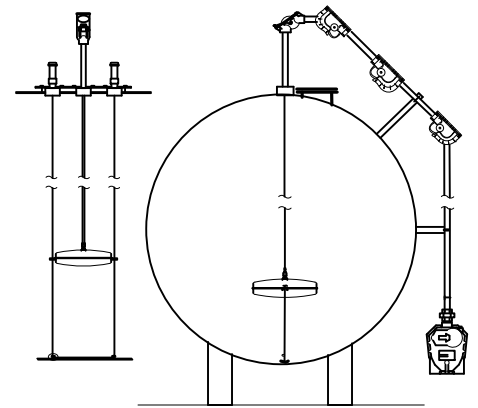
2583SK IN SERVICE KIT TOP MOUNTED (SUMP KIT)
