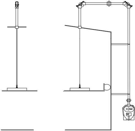
2577 INTERNAL FLOATING ROOF WITHOUT FLOAT WELL
