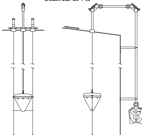
2570-TURB TURBULENT/AGITATED PRODUCTS, GROUND READING
