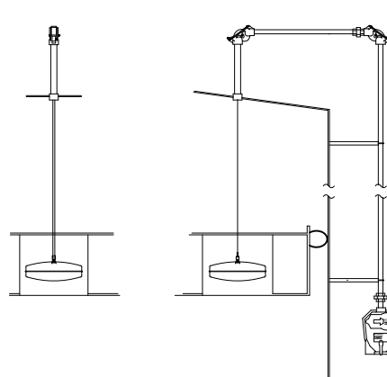
2576 INTERNAL FLOATING ROOF WITH FLOAT WELL
