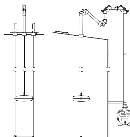
2574 CONE ROOF TANK WITH LIQUID SEAL
