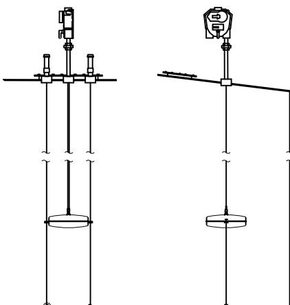
2573 CONE ROOF TANK ROOF MOUNTED
