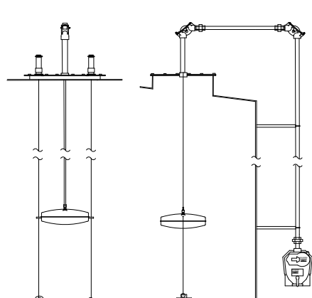
2575 IN SERVICE KIT FOR CONE ROOF TANKS
