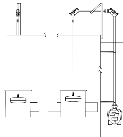
2571 EXTERNAL FLOATING ROOF TANK WITH FLOAT WELL
