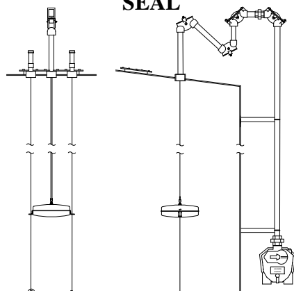
2574-HVPD HEAVY PRODUCTS WITH LIQUID SEAL
