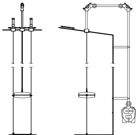
2572 EXTERNAL FLOATING ROOF WITHOUT FLOAT WELL
