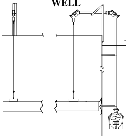
2572 EXTERNAL FLOATING ROOF WITHOUT FLOAT WELL
